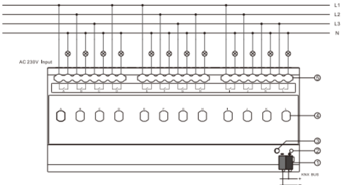
Fig.3.2(3)ARCD-12/16.S
