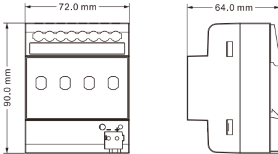
Fig.3.1(1)ARCD-04/16.S
