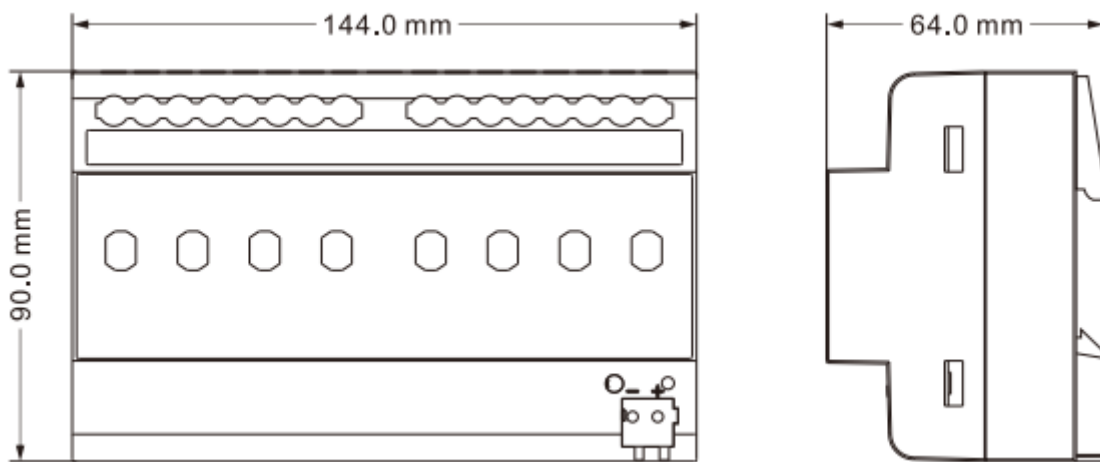
Fig.3.1(2)ARCD-08/16.S
