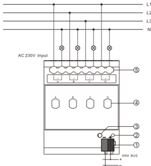
Fig.3.2(1)ARCD-04/16.S
