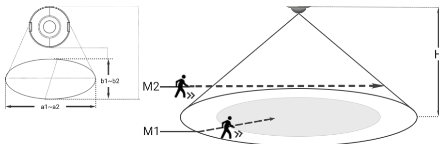
Fig.3.3.2(1)Installation diagram of HM-PIR-01
