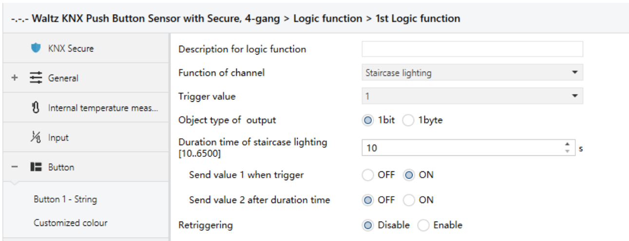
Fig.5.6.7 “Staircase lighting” parameter window
