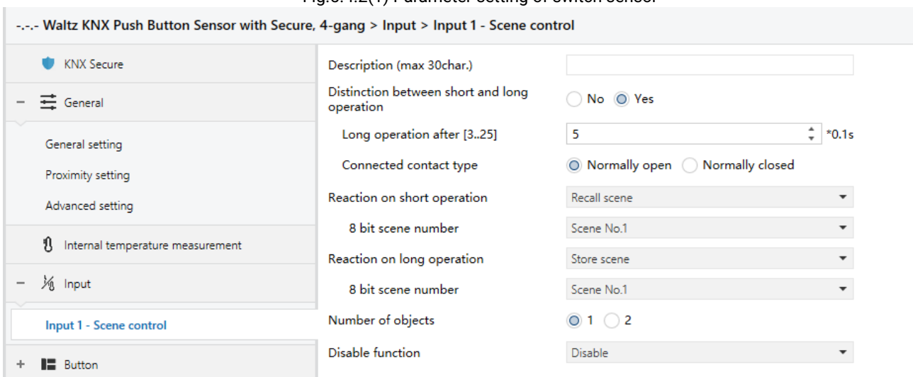
Fig.5.4.2(2) Parameter setting of scene control
