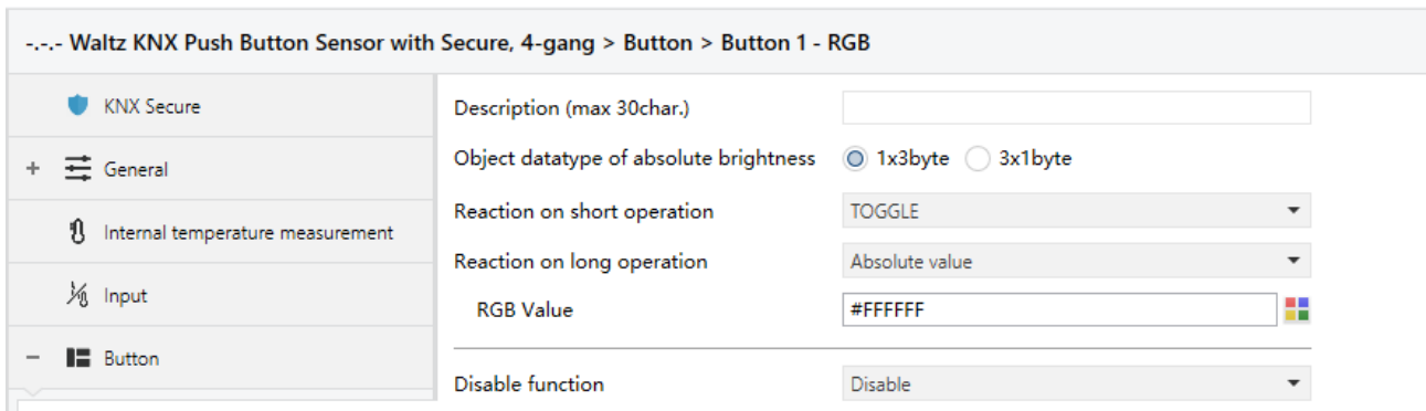
Fig.5.5.3 Parameter setting of RGB lighting function
