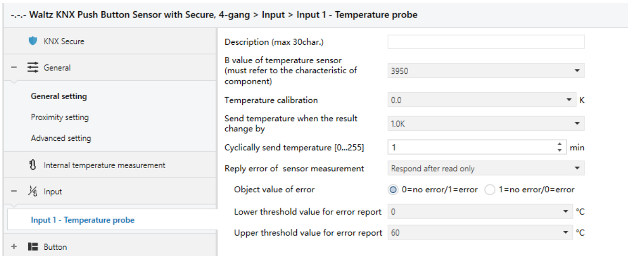
Fig.5.4.1 Parameter setting of temperature probe
