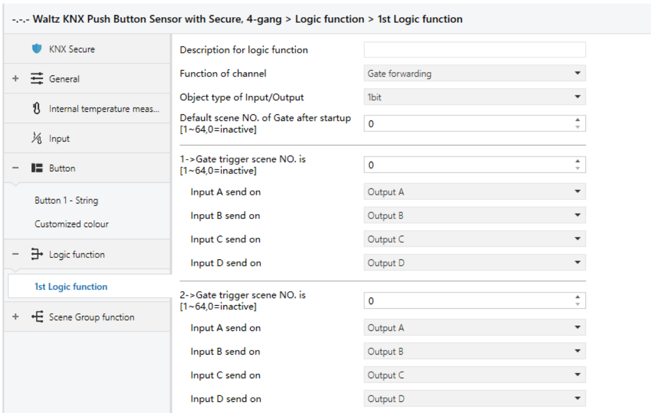
Fig.5.6.2 “Gate forwarding” parameter window
