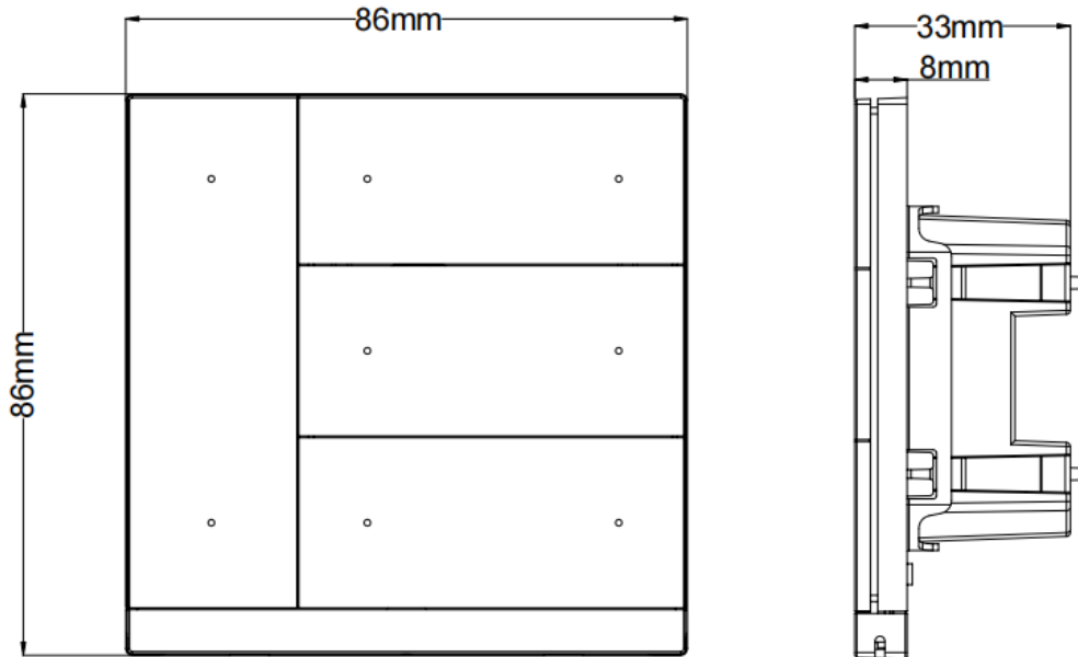
Panel dimension
