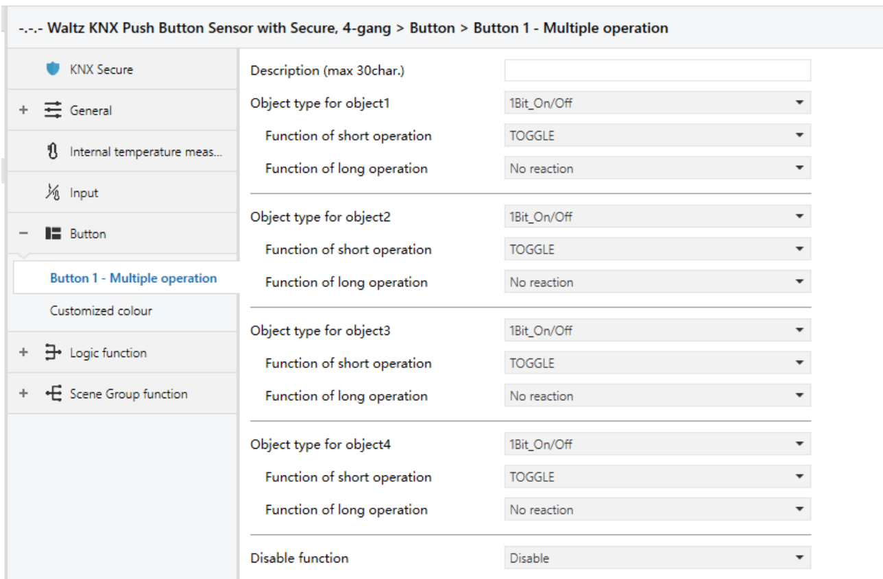
Fig.5.5.10 Parameter setting of multiple operation function
