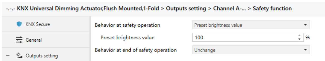
Fig.5.3.3.5 "Safety function" parameter window
