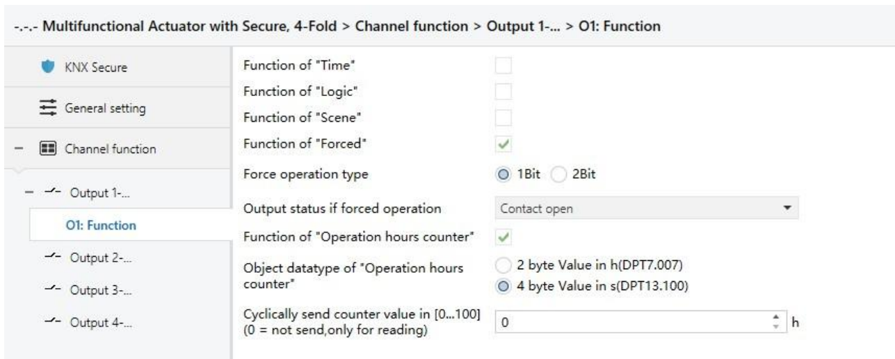
Fig. 4.4.6 Parameter window “Ox: Operation hours counter”
