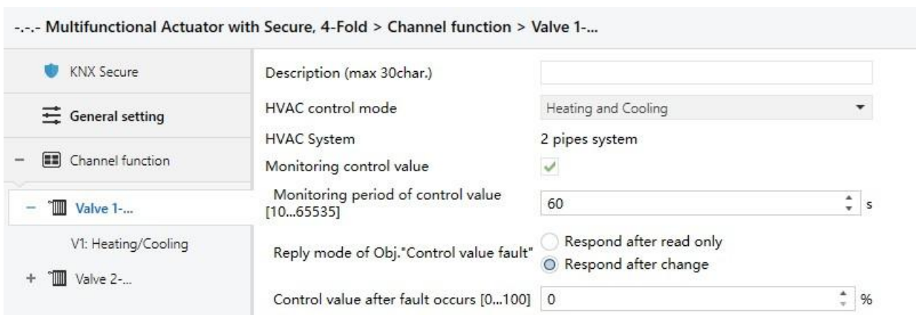
Fig. 4.9(4) Parameter window“Valve X General--Heating and Cooling (2-pipes)”
