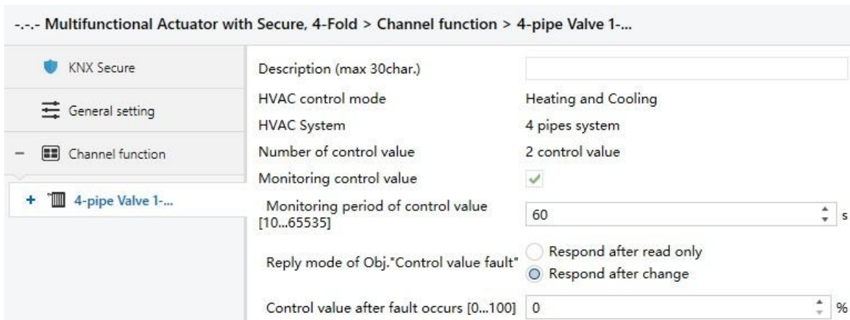
Fig. 4.9(5) Parameter window "4-Pipe Valve X General--Heating and Cooling (4-pipes)"
