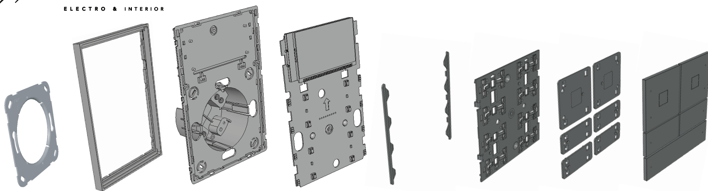
g Base Support h Face frame f Base e PCB d Light bar c First Key holder b Second Key holder a Warp switch
