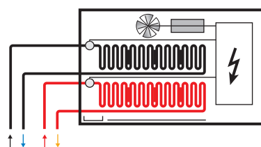
fan coil a 4 tubi
