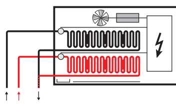
fan coil a 3 tubi
