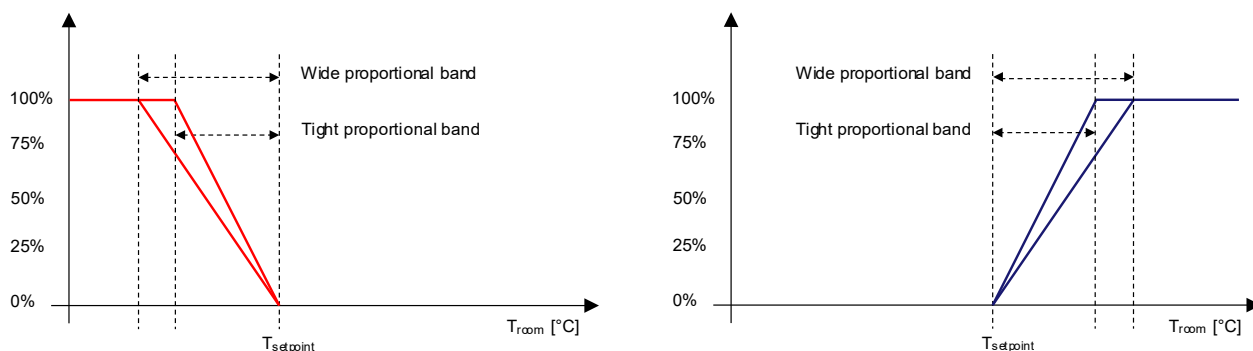
Fig. 39: Continuous PI Control Proportional Band Widths
