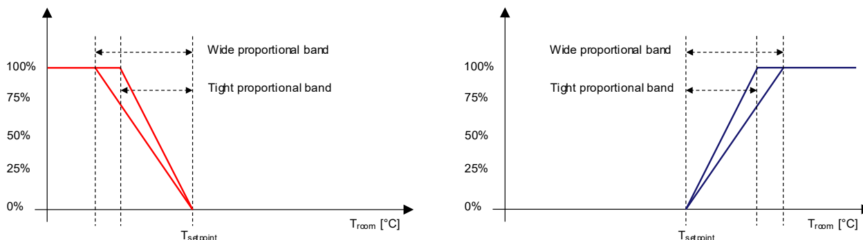
Fig. 63: Fan Controller Proportional Control
