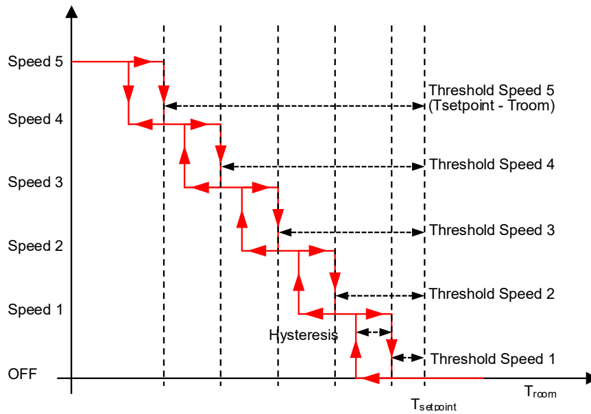
Fig. 60: Fan Controller 2-Points Control Cycle for Heating
