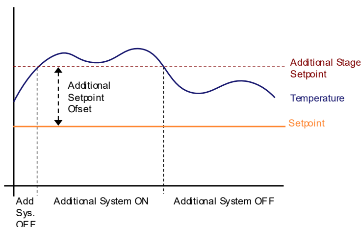
Fig. 54: PI Continuous Graph for Additional Cooling Control
