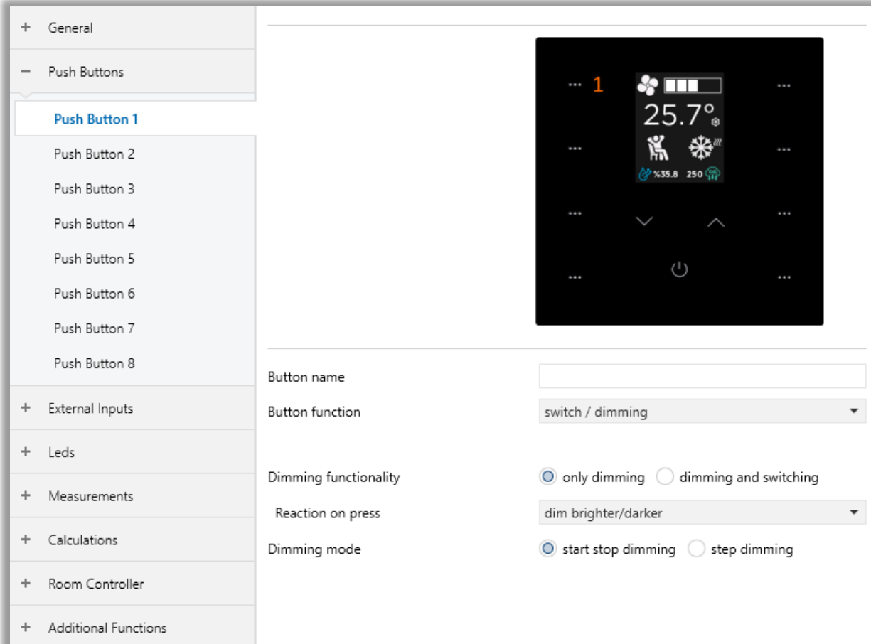
Fig. 13: Switch/Dimming Function Configuration Page
