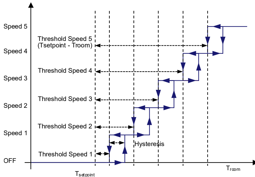
Fig. 61: Fan Controller 2-Points Control Cycle for Cooling
