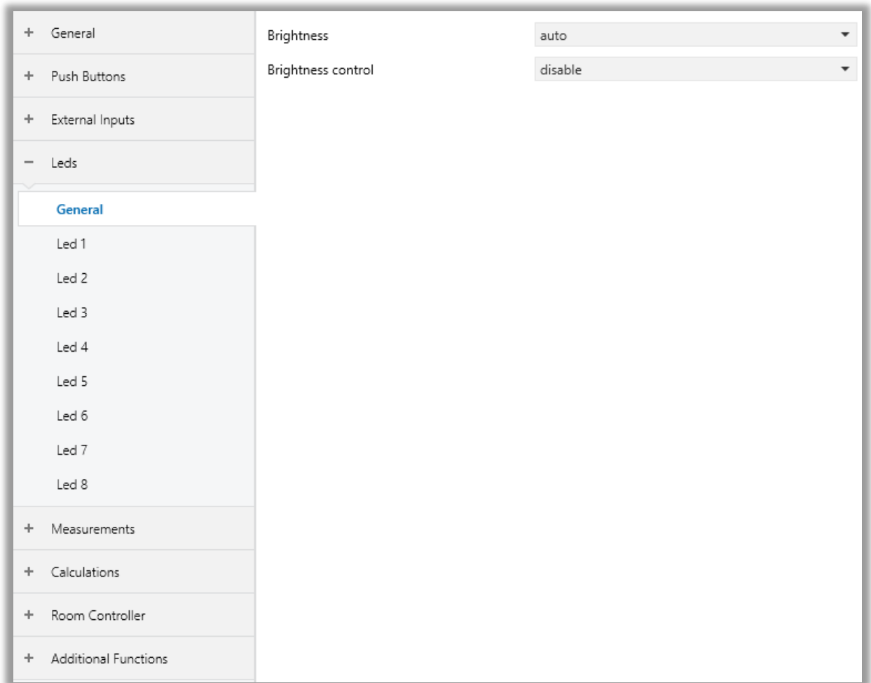
Fig. 28: LEDs General Page
