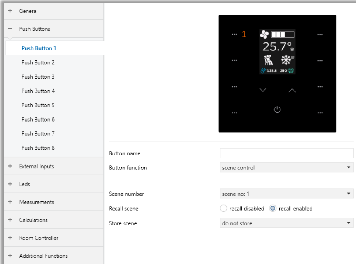
Fig. 16: Scene Control Function Configuration Page
