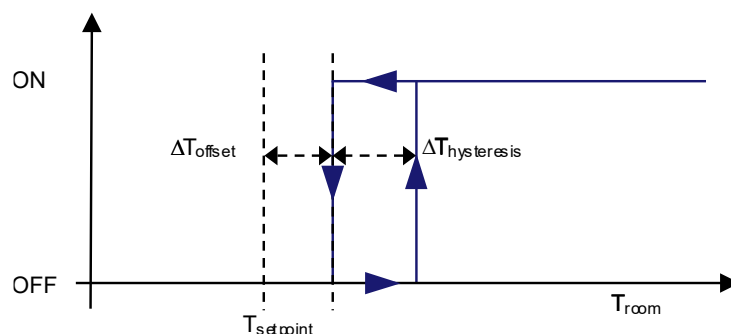
Fig. 53: 2 – Points Hysteresis Cycle for Additional Cooling Control
