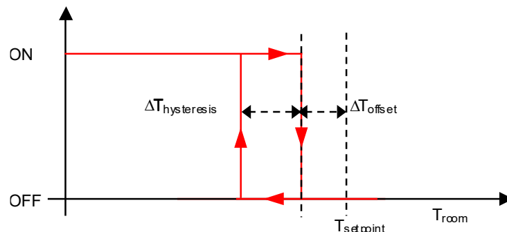
Fig. 47: 2 – Points Hysteresis Cycle for Additional Heating Control
