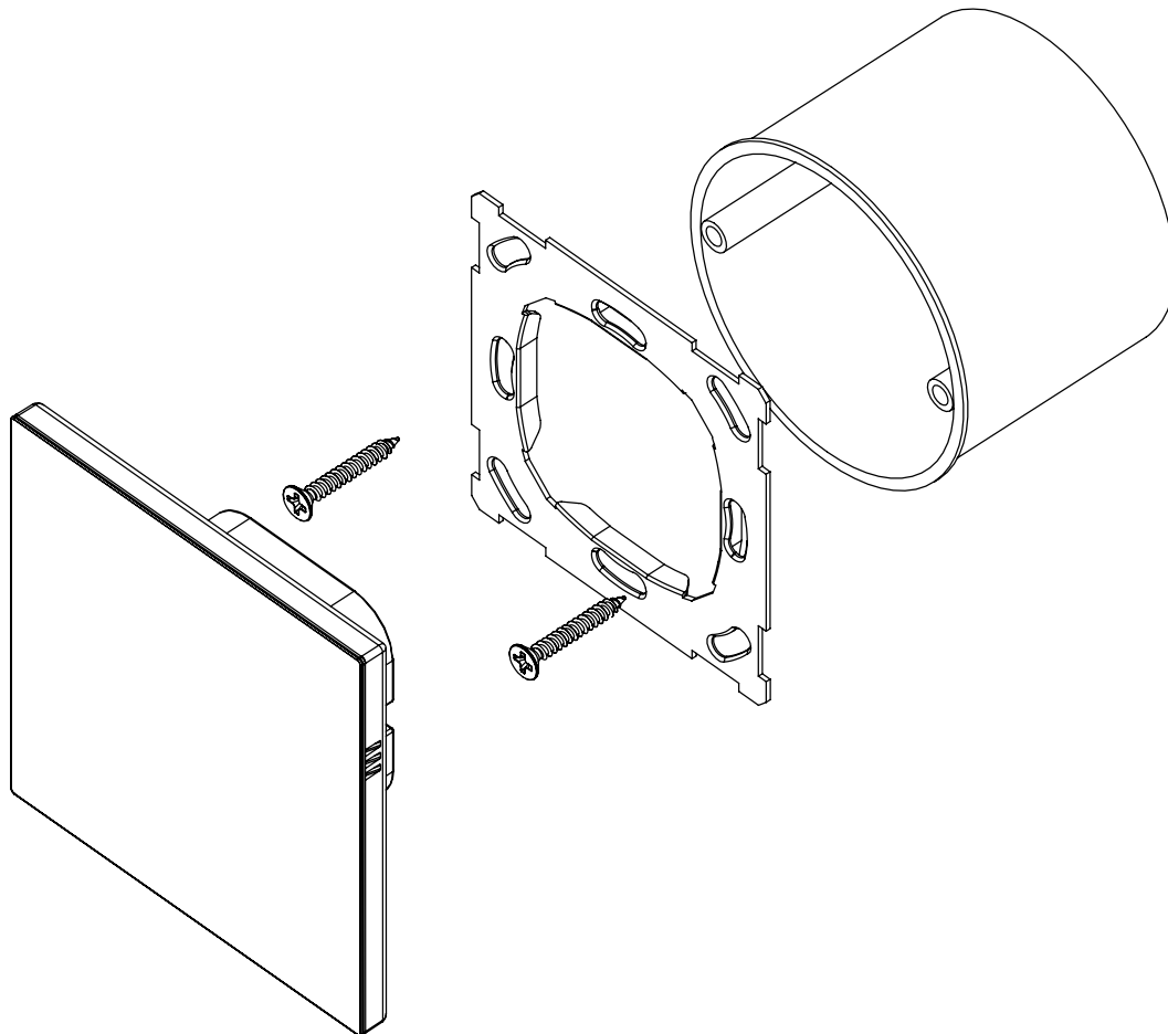
Fig. 8: Mounting the Flush Mounting Box
