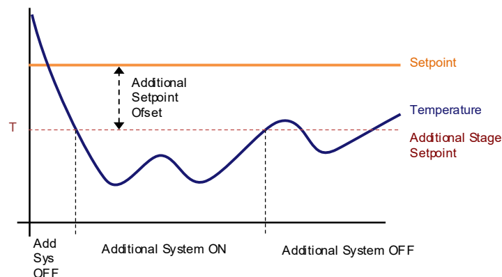
Fig. 48: PI Continuous Graph for Additional Heating Control
