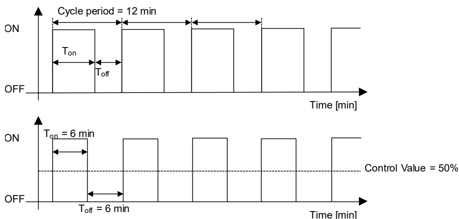
Fig. 40: PWM Control Sampling
