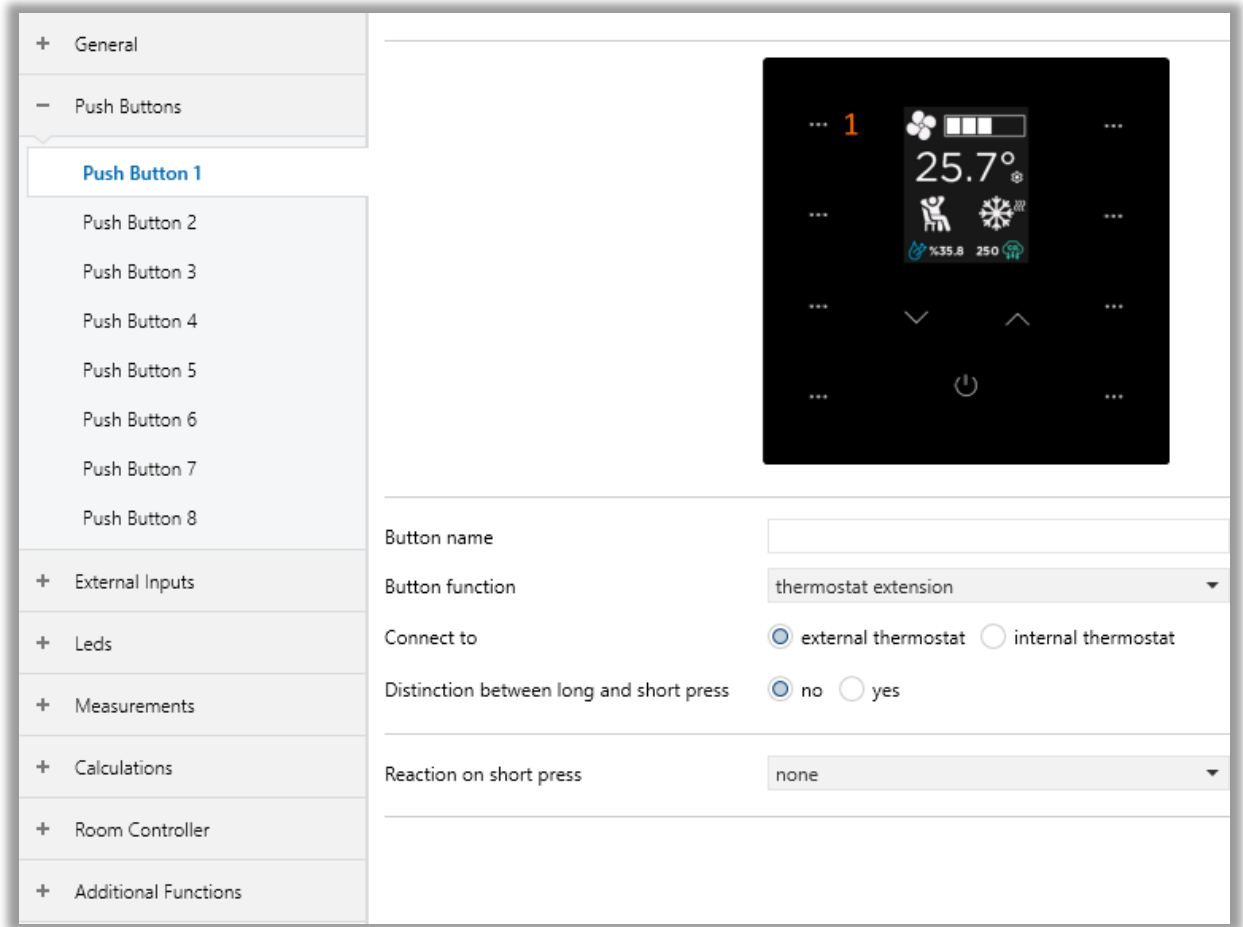
Fig. 22: Thermostat Extension Configuration Page
