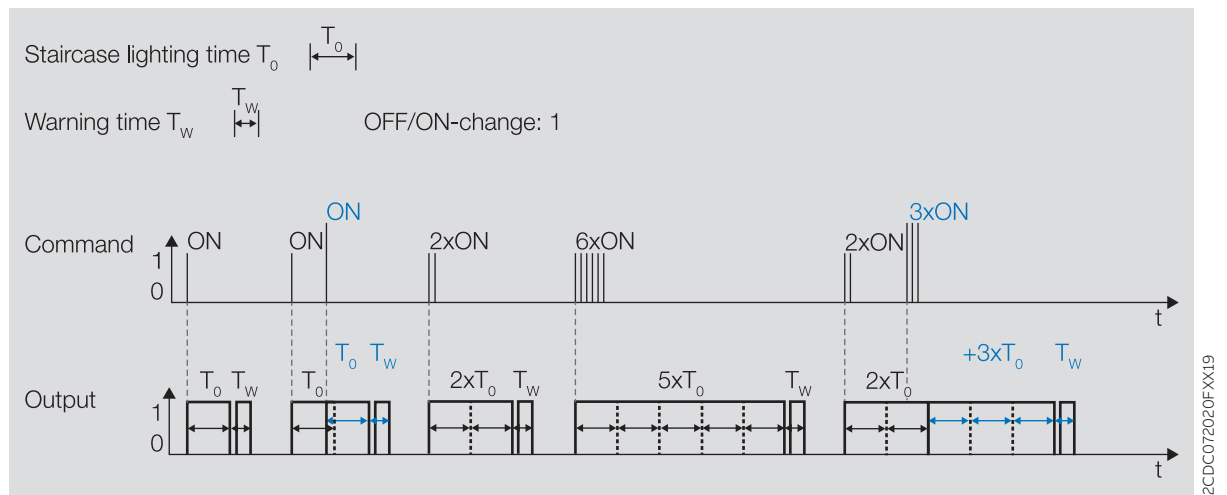
Fig. 20: Extending staircase lighting time (retriggering/pumping)
