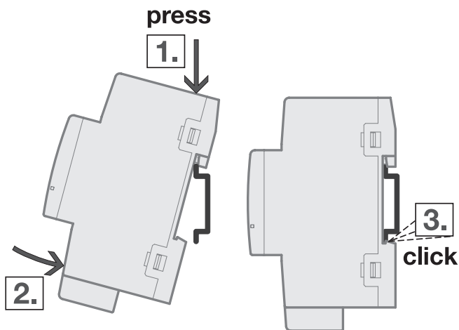
Fig. 21: Mounting on mounting rail
