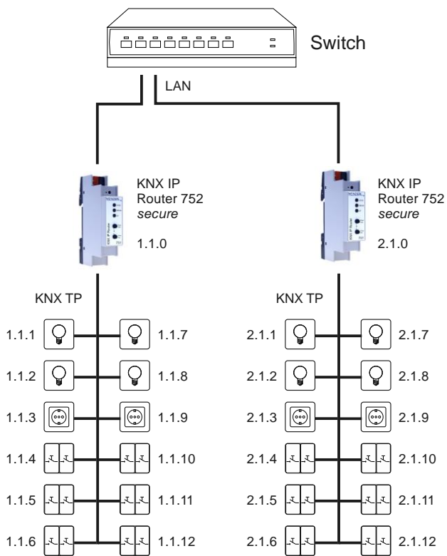
KNX IP Router as line coupler
