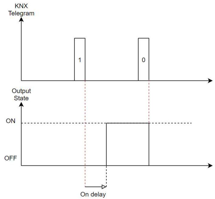
Figure 5 On delay
