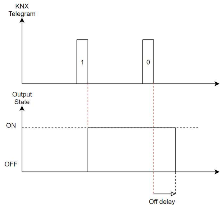
Figure 6 Off delay
