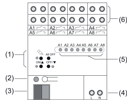
Figure 1: Device components front view
