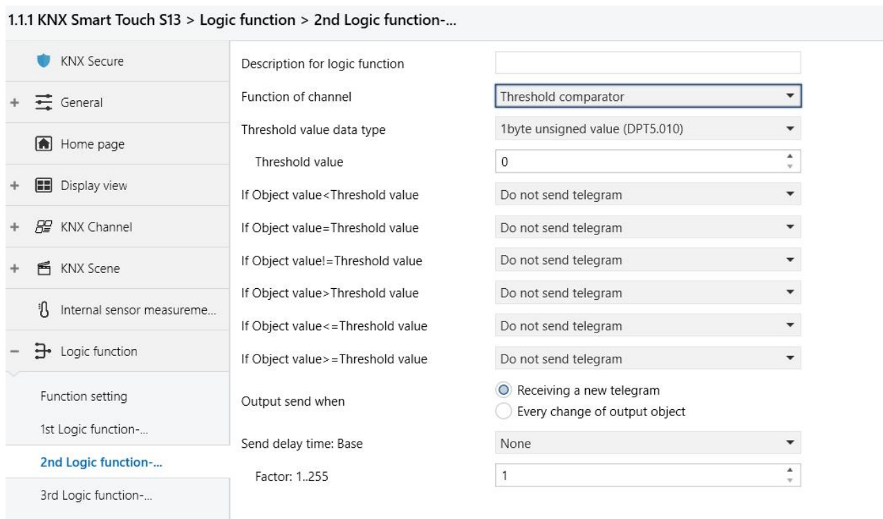
Fig.5.7.3 "Logic function_Threshold comparator"parameter window
