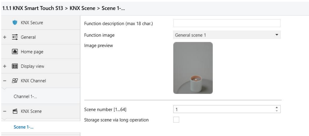
Fig.5.12(2) "Scene X"parameter window
