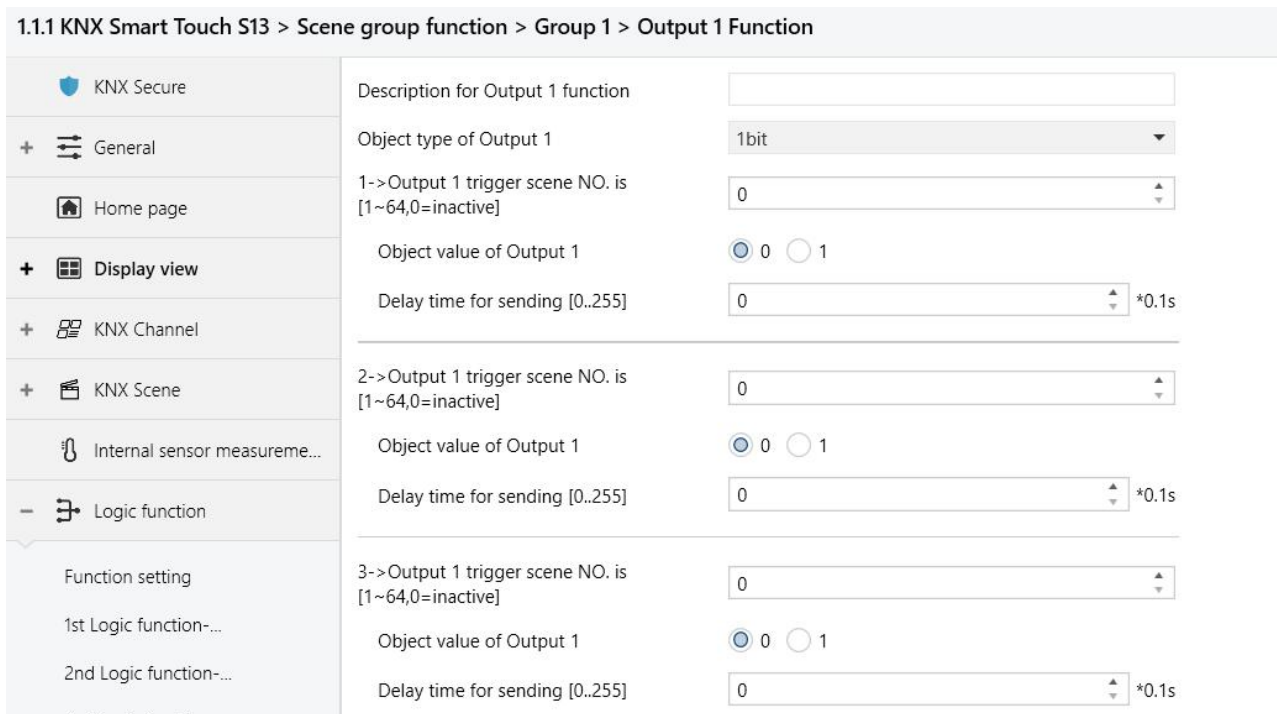
Fig.5.8(3) "Output Y function"parameter window
