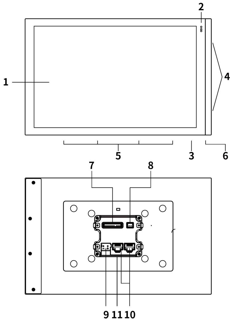
Fig.3.2.1 KNX Smart Touch S13 structural diagram
