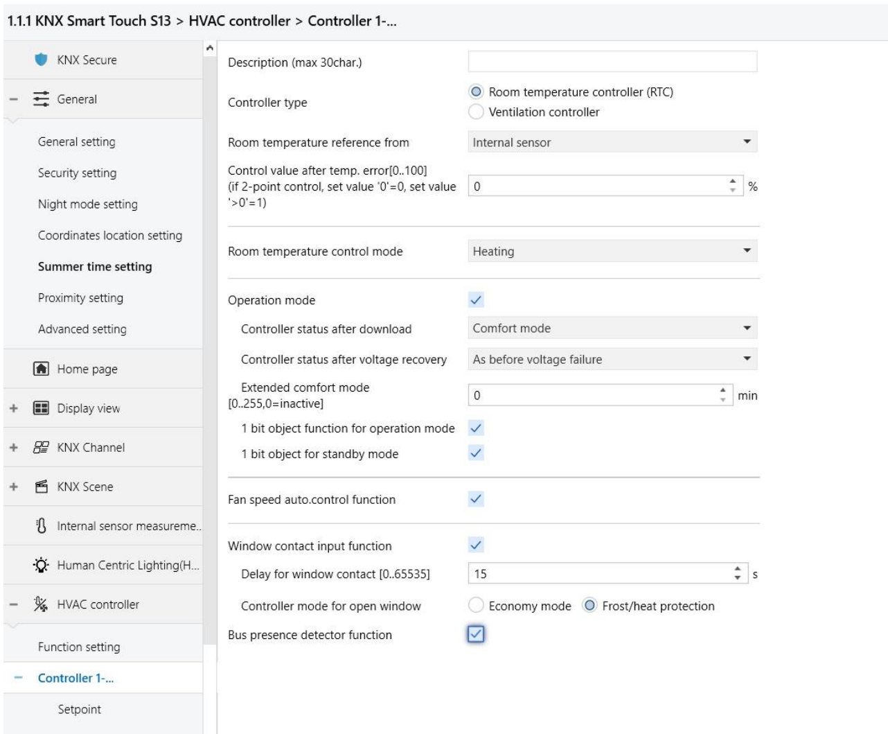
Fig.5.3.1 "Controller x-Room temperature controller(RTC)"(x=1~6) parameter window
