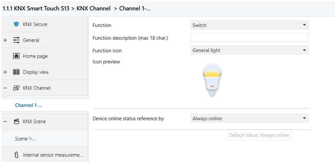
Fig.5.11.1 "Channel X"parameter window
