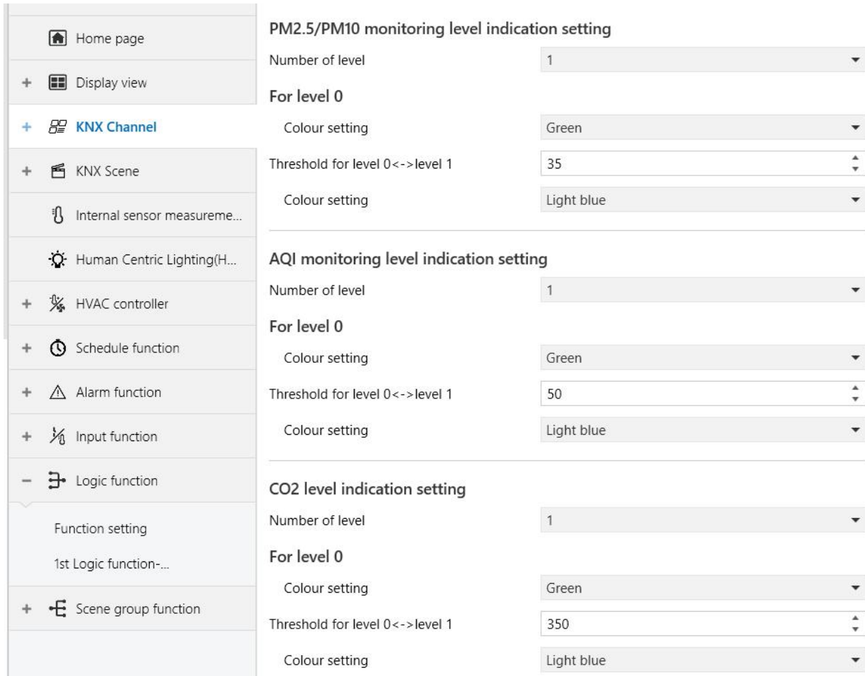
Fig.5.11 "KNX Channel"parameter window
