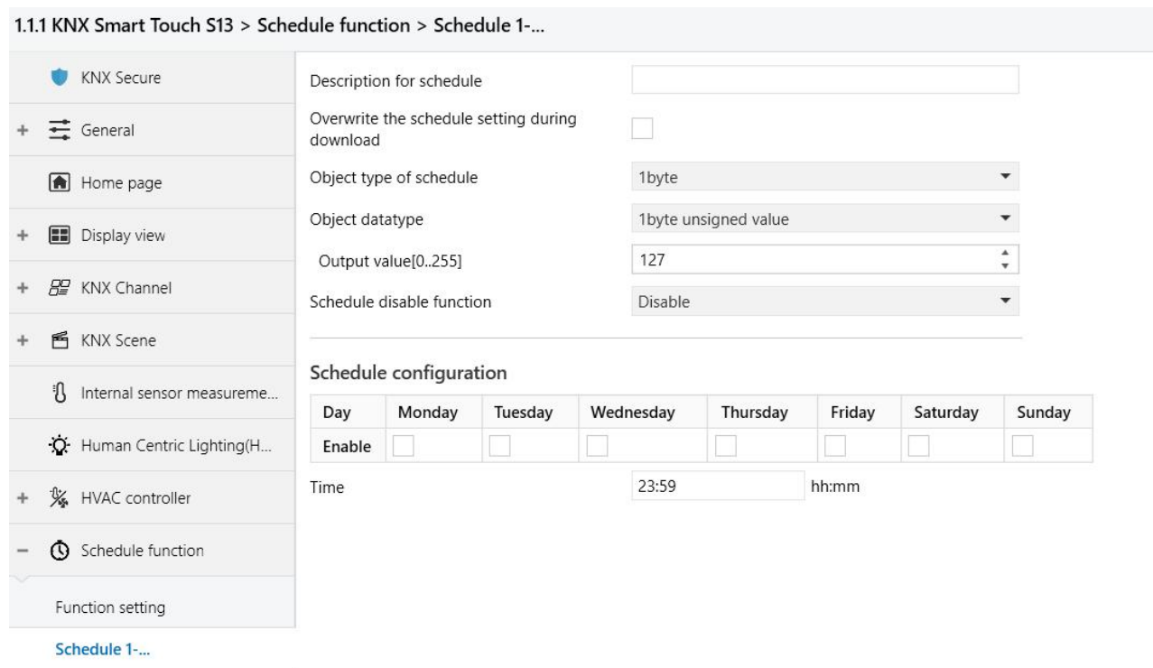
Fig.5.5.1 "Schedule X"parameter window
