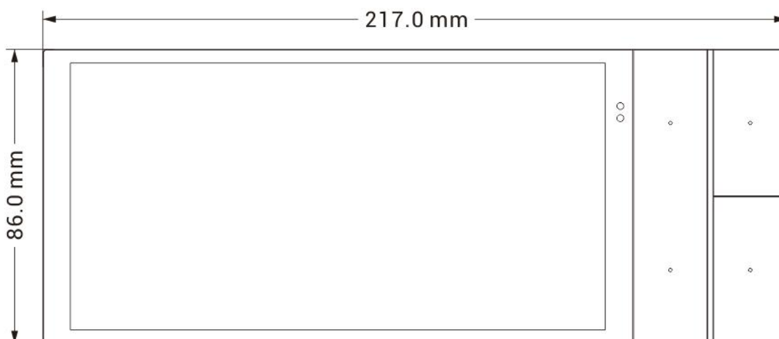
Fig.3.1.1(2) KNX Smart Touch S7 with S7 Extension Sub Panel, 4 buttons
