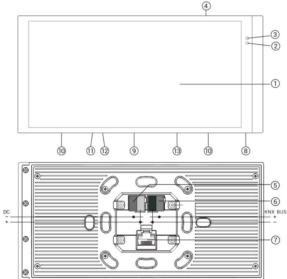
Fig.3.2.1 KNX Smart Touch S7 structural diagram
