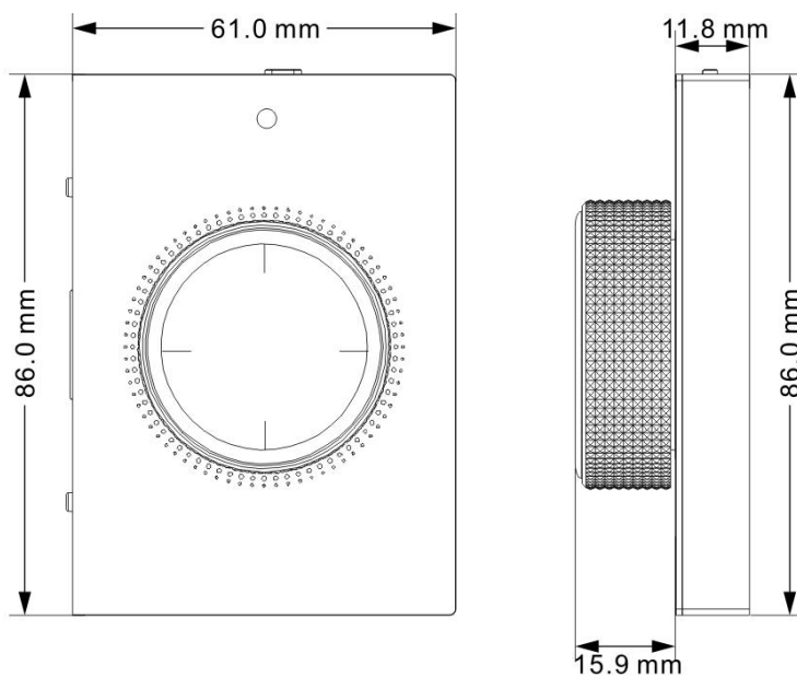
Fig.3.1.3 Extension Sub Panel, 4 buttons with Rotary
