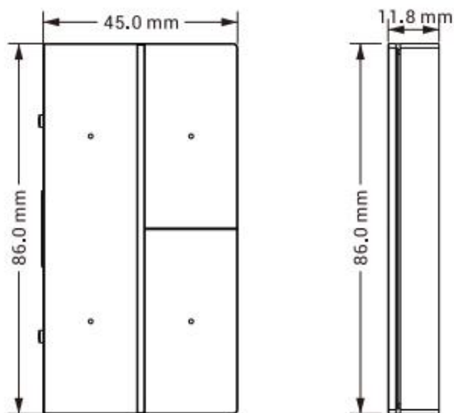
Fig.3.1.2 S7 Extension Sub Panel, 4 buttons
