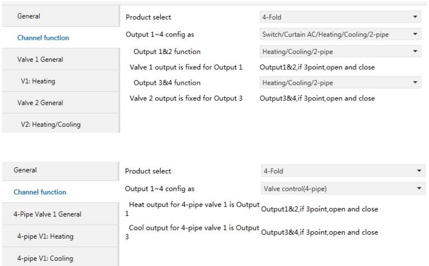
Fig. 4.26 Parameter window Channel function--valve type”
