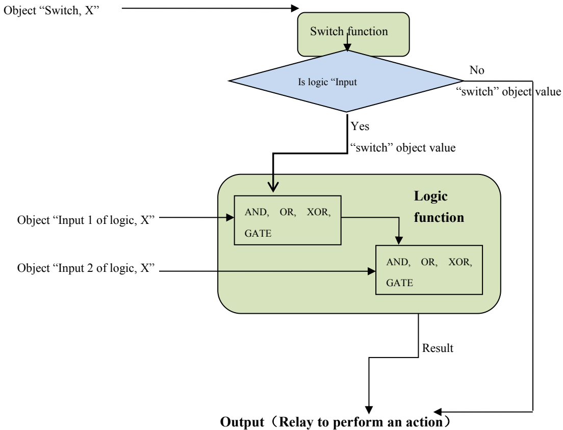
Fig. 4.4 switch and logical function diagram
