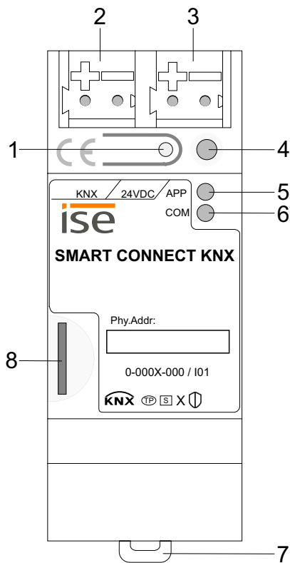
Figure 4: Front
