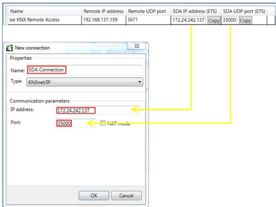
Figure 18: Manual KNX/IP interface configuration for ETS prior to ETS4.2
