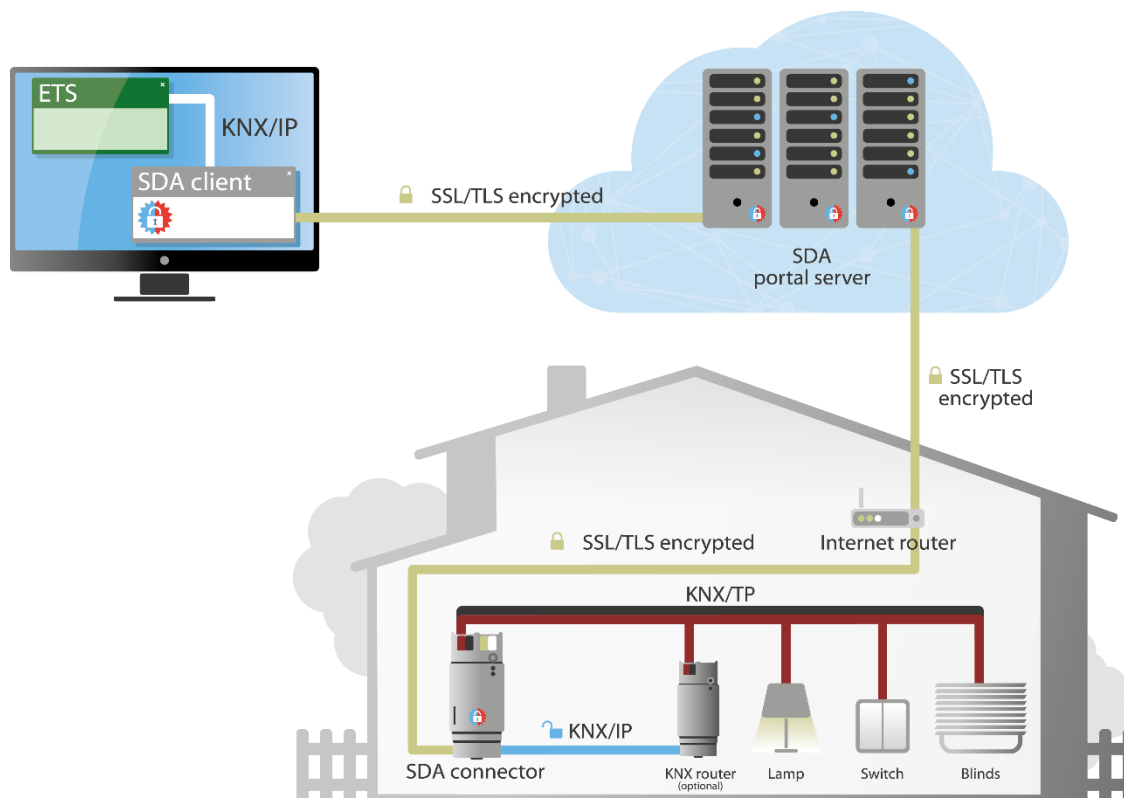
Figure 3: Secure access to the KNX installation via "Secure Device Access"
