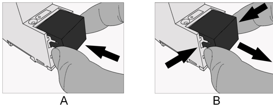
Figure 27: Mounting / removing cover cap
