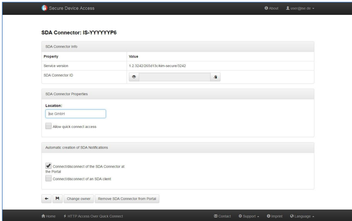
Figure 8: Displaying and changing properties of an SDA connector
