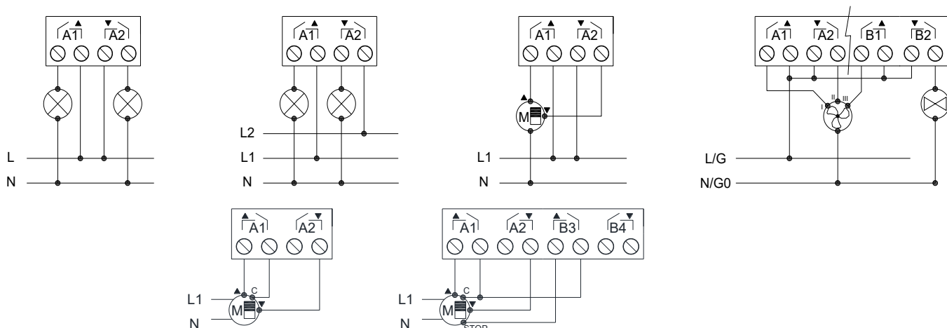
Figure 2: Wiring example (from top to bottom and left to right): 2 loads, 2 loads connected to different phases, shutter channel, 2-pipe fan coil three-speed fans, open/close valve, one shutter with 2 dry contacts and one shutter with 3 dry contacts
