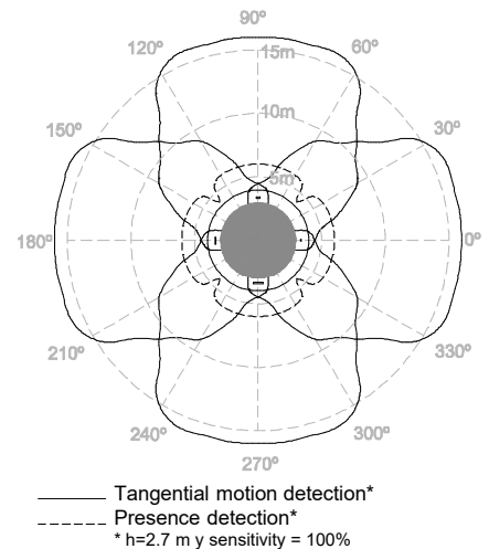
Figure 3. Detection sectors
