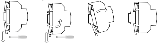
Removing RailQUAD 8 v2 from DIN rail:
