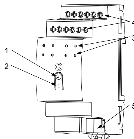
Figure 1: RailQUAD 8 v2
