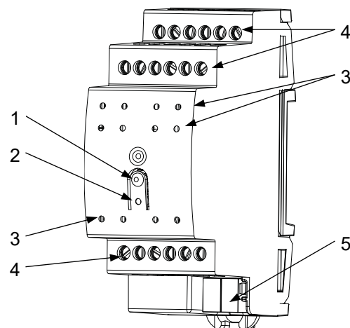
Figure 1 : RailQUAD 12
