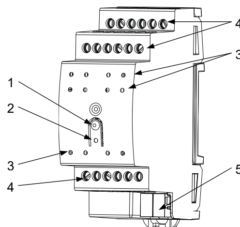
Figure 1: RailQUAD 12
