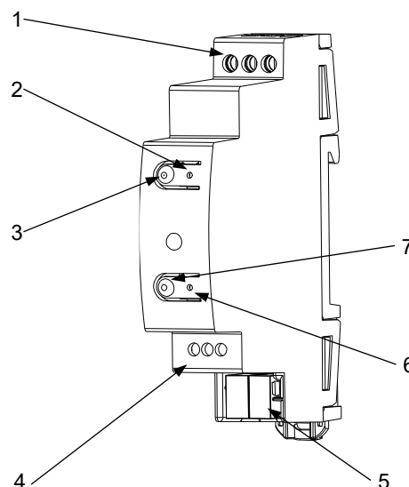
Figure 1: MicroBOX 12
