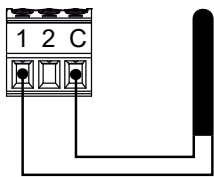
Zennio temperature probe.
