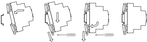
Removing KLIC-MDI from DIN rail:
