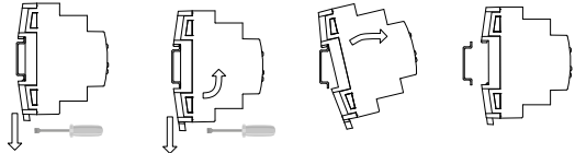
Removing KLIC-MDI from DIN rail:
