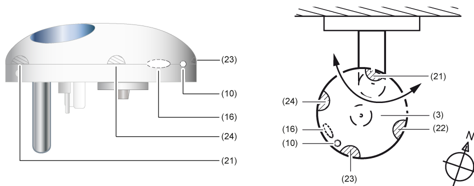
Figure 8: Operating elements
