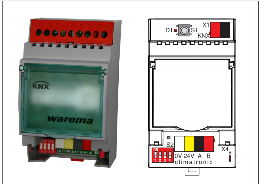
Fig. 3 KNX Gateway
