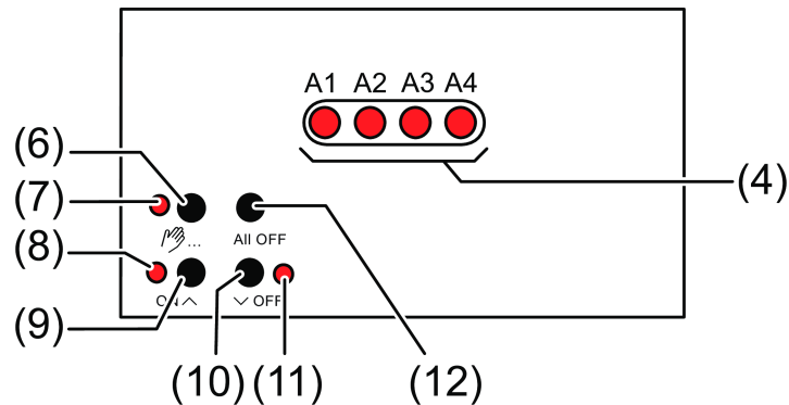
Figure 5: Operating elements
