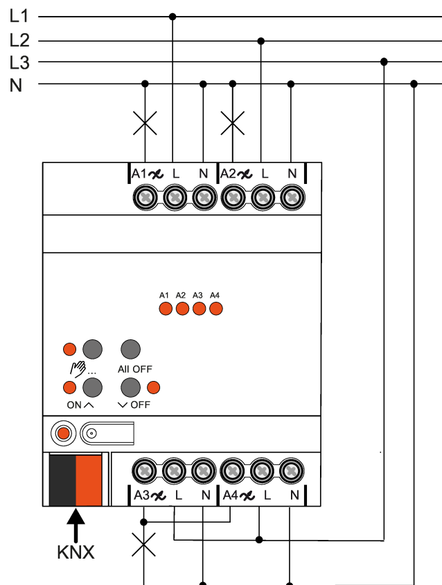
Figure 4: Comfort variant of the device connection with dimmer outputs switched in parallel (connection example)
