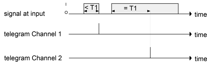
Figure 40: Example of operating concept "Channel 1 or Channel 2"
