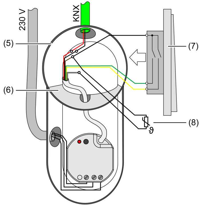
Figure 5: Mounting example in electronic appliance box with partition wall, series push-button and NTC temperature sensor
