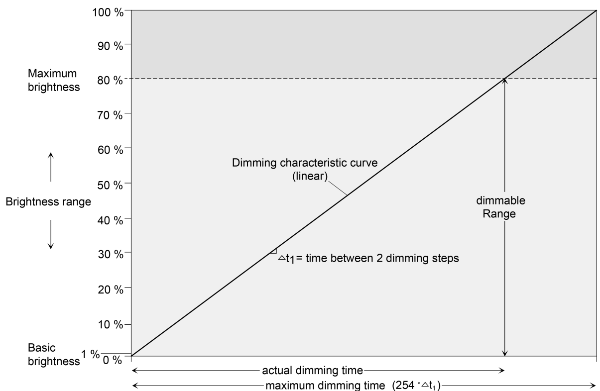
Figure 9: Linear dimming characteristic as an example with basic brightness and maximum brightness
