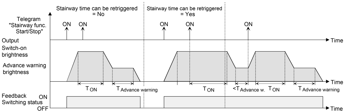
Figure 18: Switch-on behaviour of the staircase function with soft functions (as an example with minimum brightness = 0 %)
