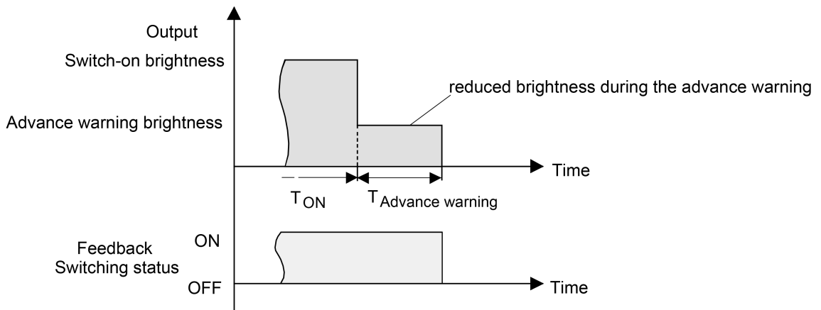
Figure 21: The pre-warning function of the staircase function without soft OFF function
