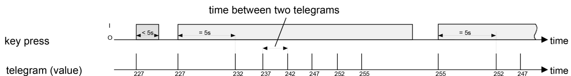
Figure 34: Example of value adjustment without value range overflow
