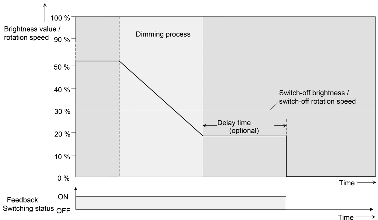
Figure 16: Dimming and switching behaviour of the automatic switch-off function
