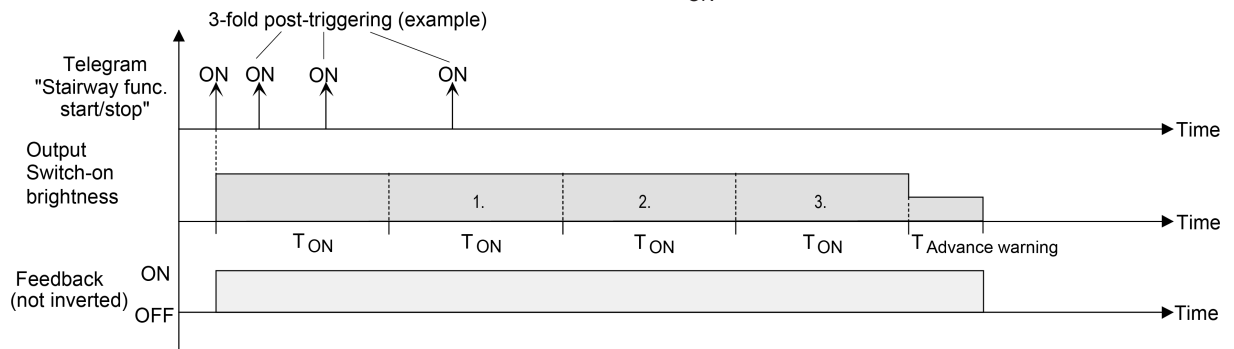
Figure 25: Time extension of the staircase function
