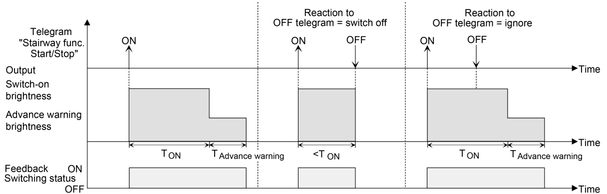
Figure 19: Switch-off behaviour of the staircase function without soft functions
