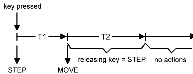
Figure 30: Operating concept "short – long – short"
