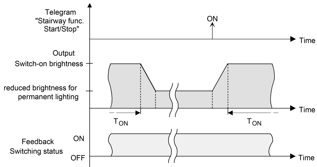
Figure 24: The continuous lighting of the staircase function with soft OFF functions
