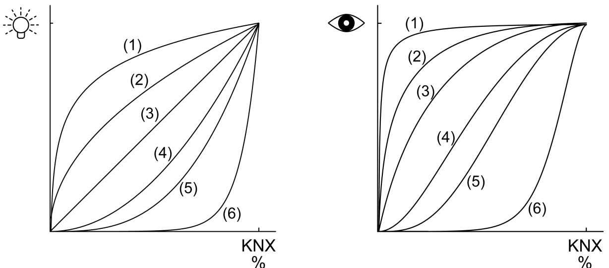
Figure 8: Dimming characteristics in the value range
