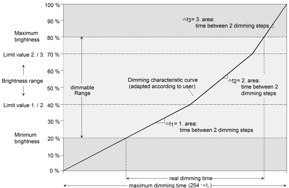
Figure 12: User-defined dimming characteristic as an example with minimum brightness and
