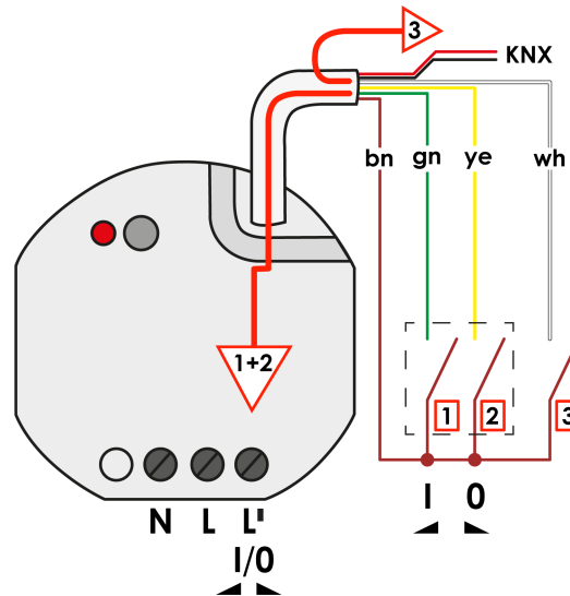
Figure 28: Functioning of the inputs when controlling the internal dimming output as dual-area operation
