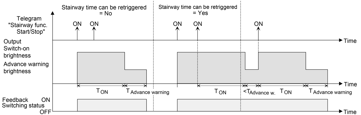
Figure 17: Switch-on behaviour of the staircase function without soft functions
