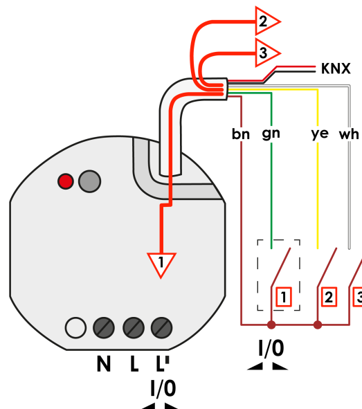
Figure 29: Functioning of inputs when controlling the internal dimming output as single-area operation
