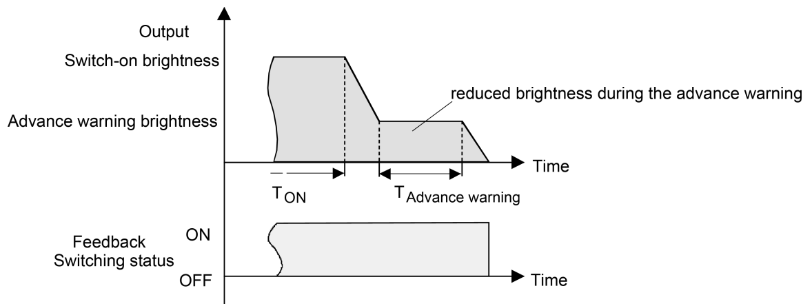
Figure 22: The pre-warning function of the staircase function with soft OFF function (as an example with minimum brightness = 0%)
