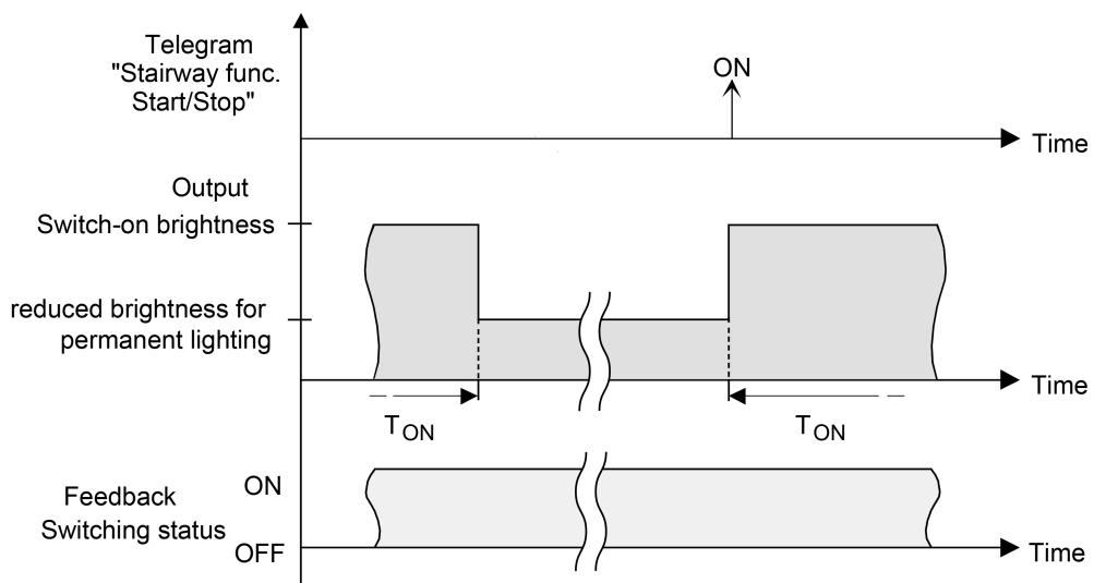
Figure 23: The continuous lighting of the staircase function without soft functions
